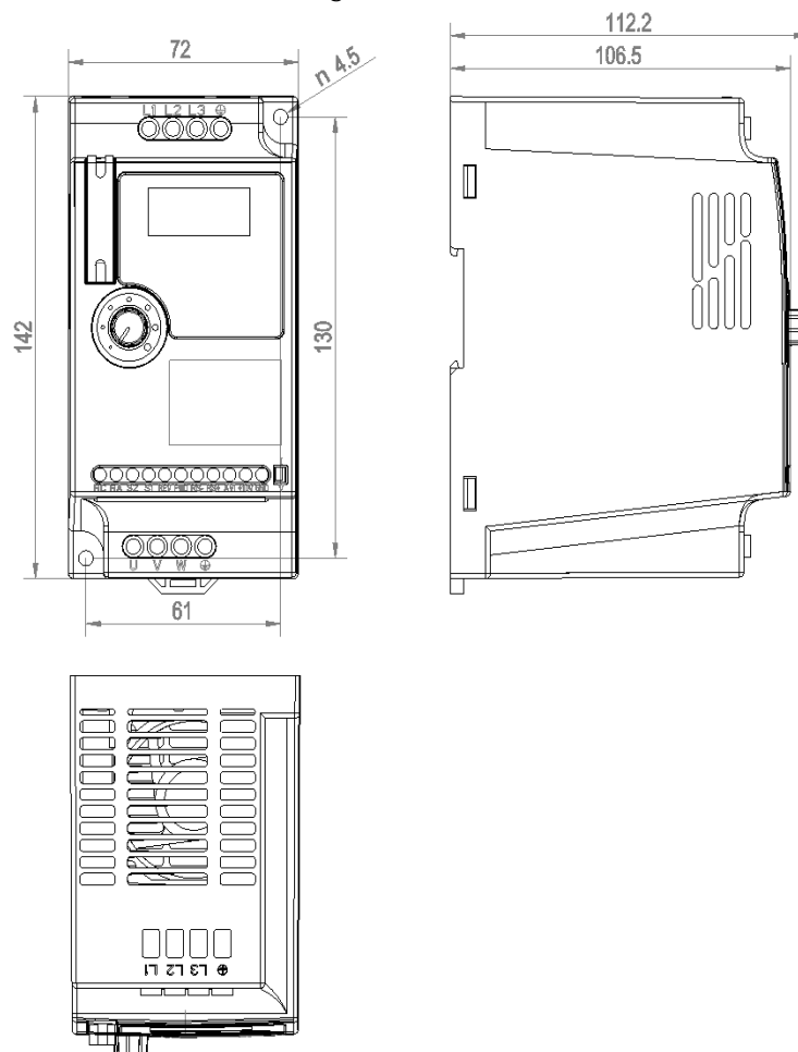
Dimensional drawing A550 Plus - 2,2kW 4T0022
