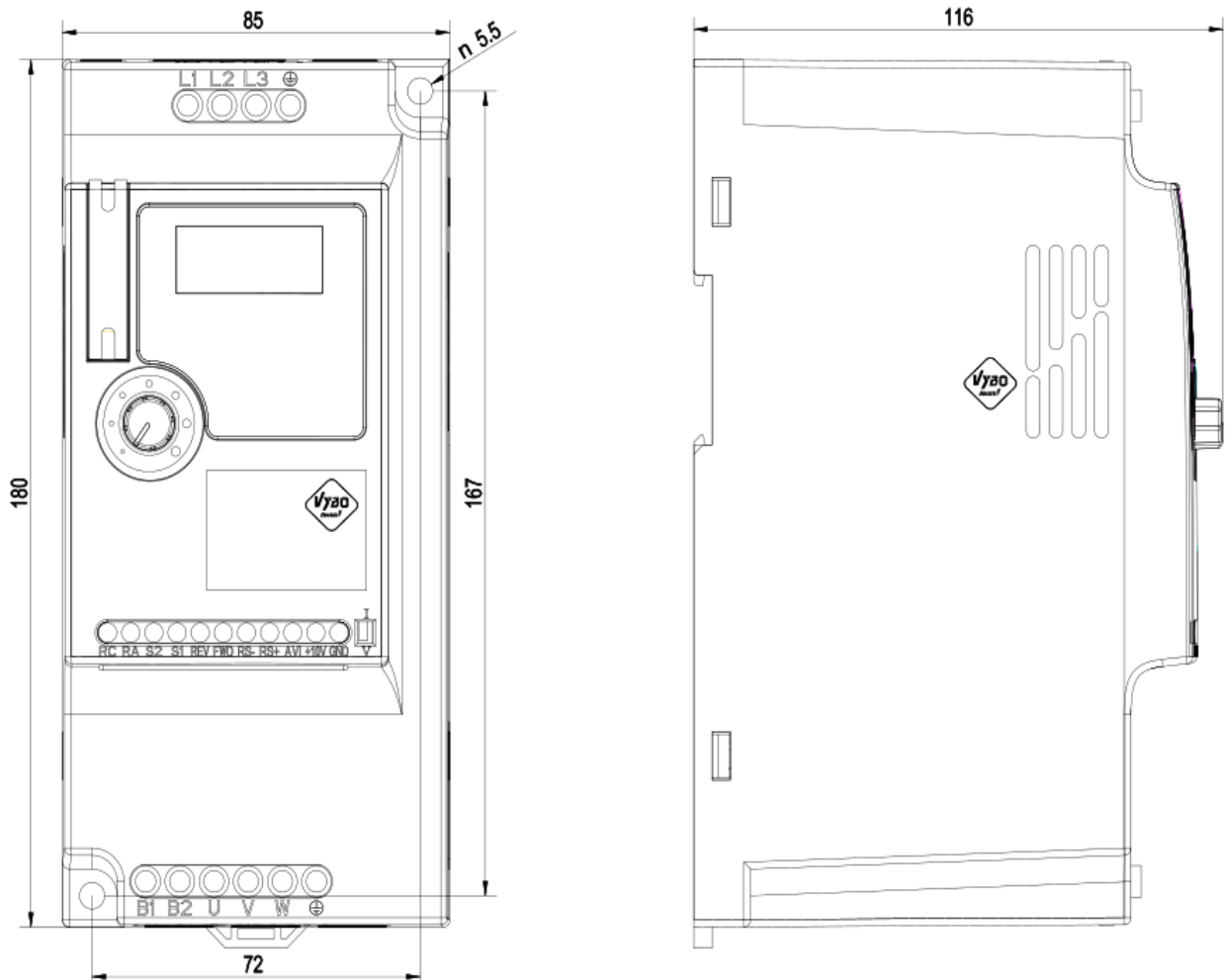
Dimensional drawing A550 Plus - 4kW 4T0040
