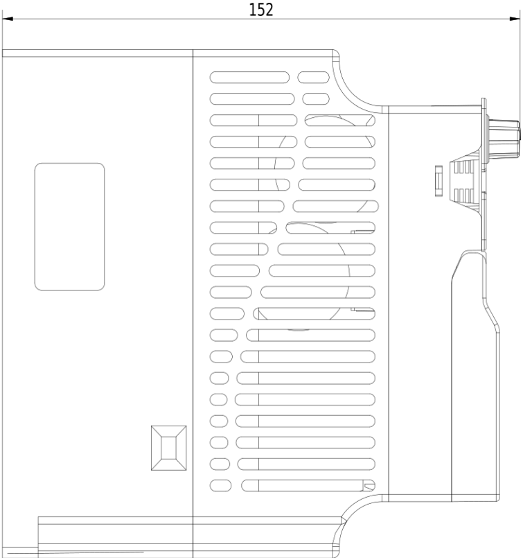
Dimensional drawing V800 - 1,5kW 2S0015
