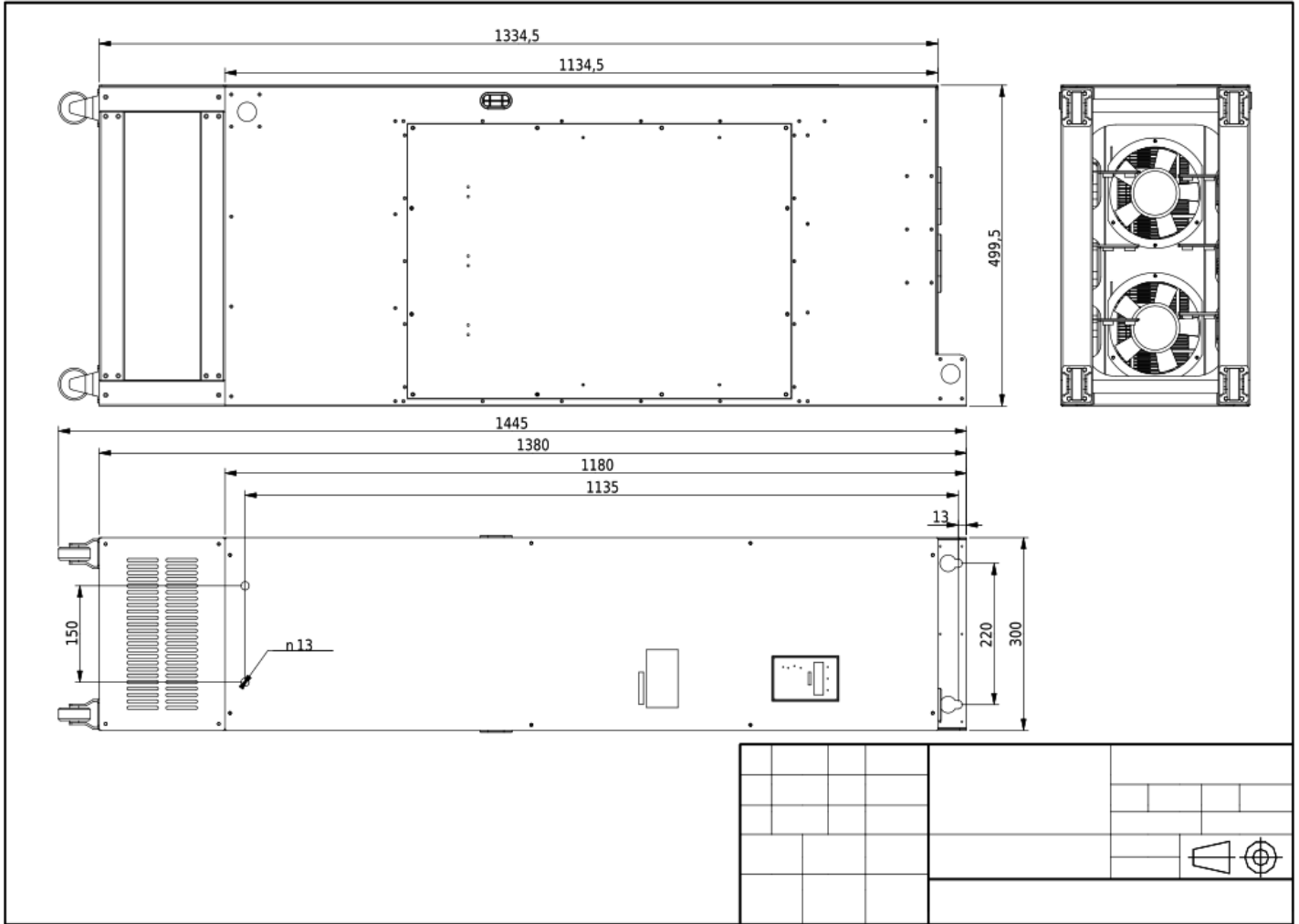
Dimensional drawing V800 - 200kW 4T2000
