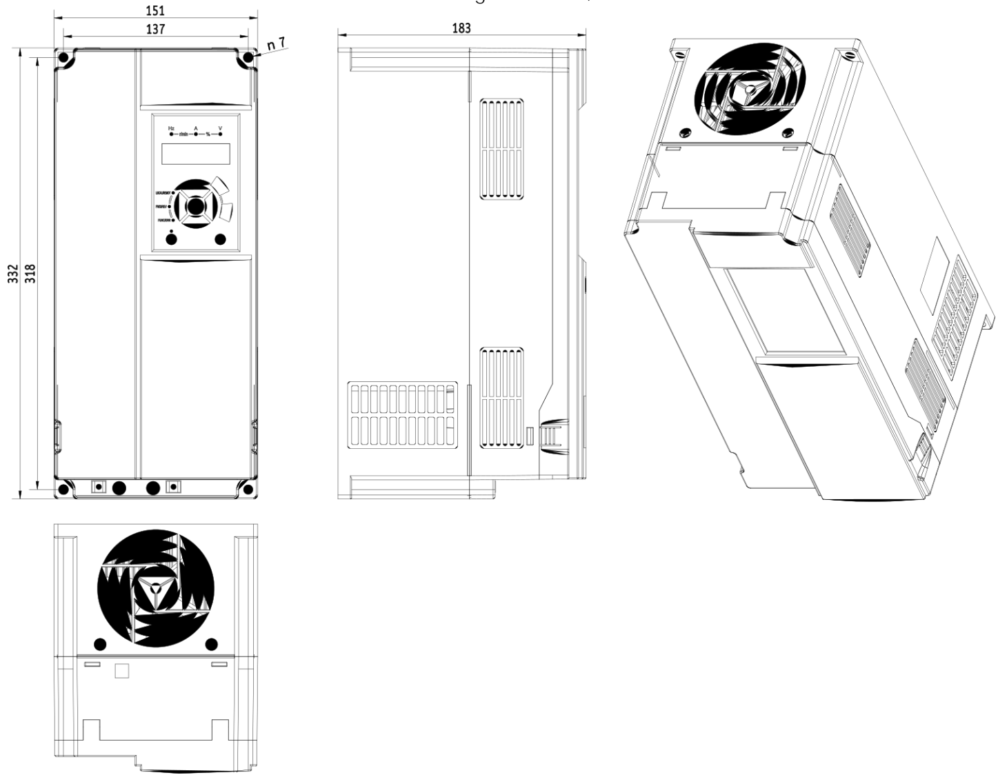
Dimensional drawing V900 - 18,5kW 4T0185
