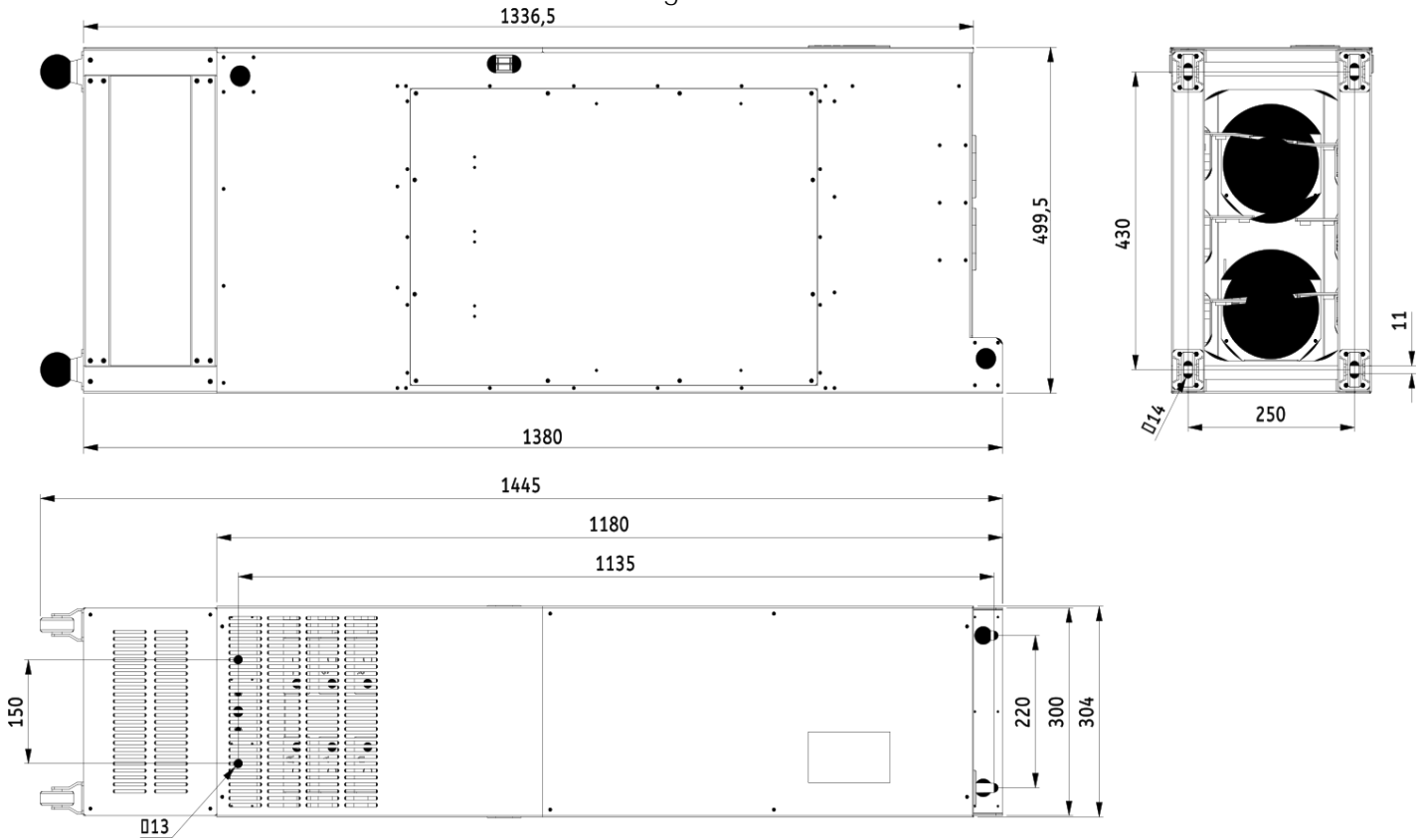
Dimensional drawing V900 - 200kW 4T2000
